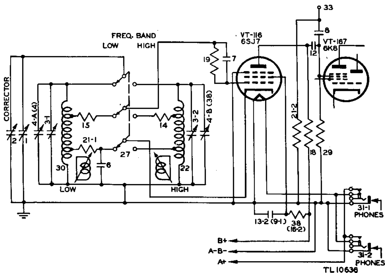
Figure 85. Frequency Meter BG-221-(7), functional diagram, variable frequency oscillator circuit.
