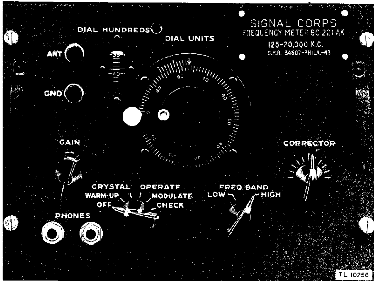
Figure 6. Frequency Meter BC-221-AK, control panel lay-out.
