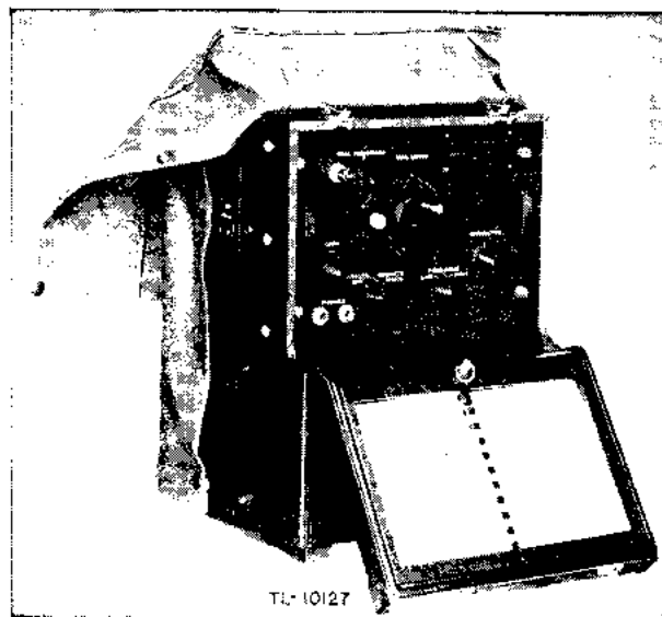
Figure 2. Frequency Meter BC-221 (Q), in wooden cabinet.
