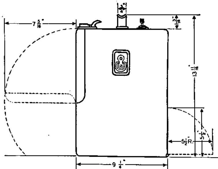
Figure 26. Frequency Meter BC-221-(3), typical dimensions, metal cabinet (subject to slight variations.)
