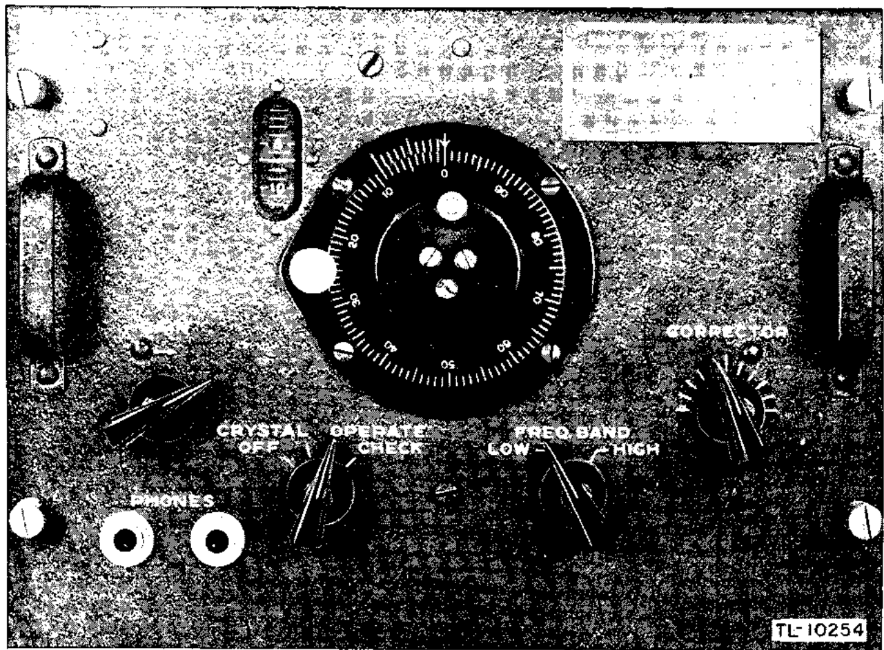
Figure 1. Frequency Meters BG-221-B, BG-221-E, BG-221-N, BG-221-Q, BG-221-AA, BG-221-AE, and BG-221-AG, control panel layout.
