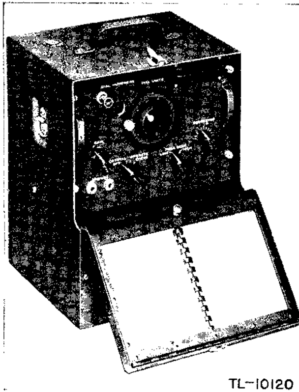
Figure 1. Frequency Meter BC-221 (Q), in metal cabinet.
