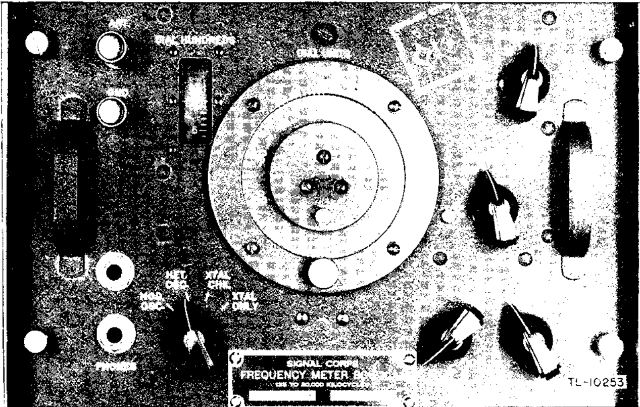
Figure 7. Frequency Meter BC-221-A7 and BC-221-A1, control panel layout.
