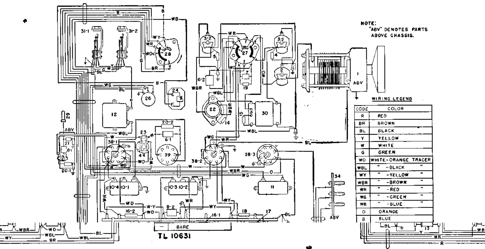
Frequency Meter BG-221-E, chassis wiring diagram.
