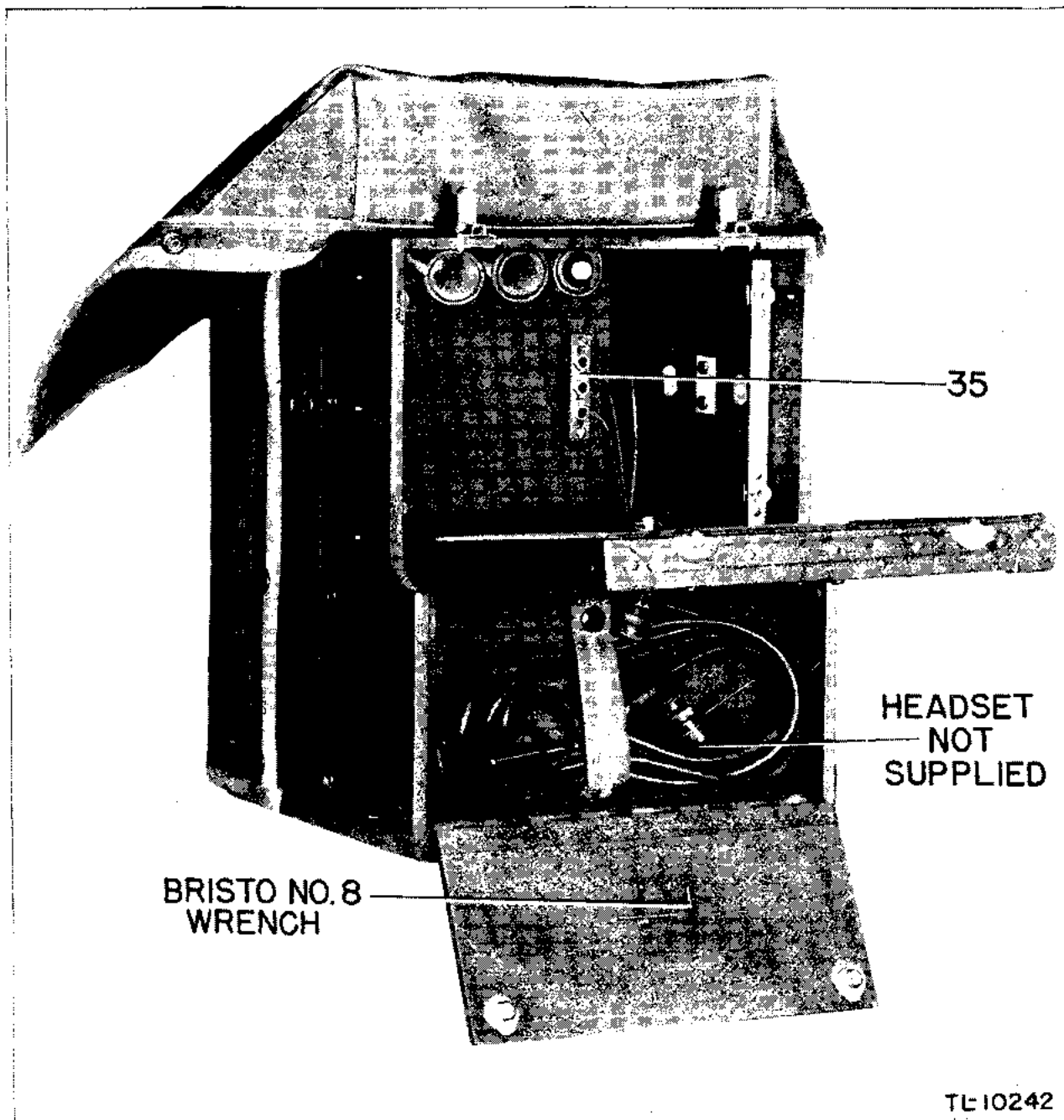
Figure 25. Frequency Meter BC-221-(C), typical wooden cabinet, showing headset compartment.
