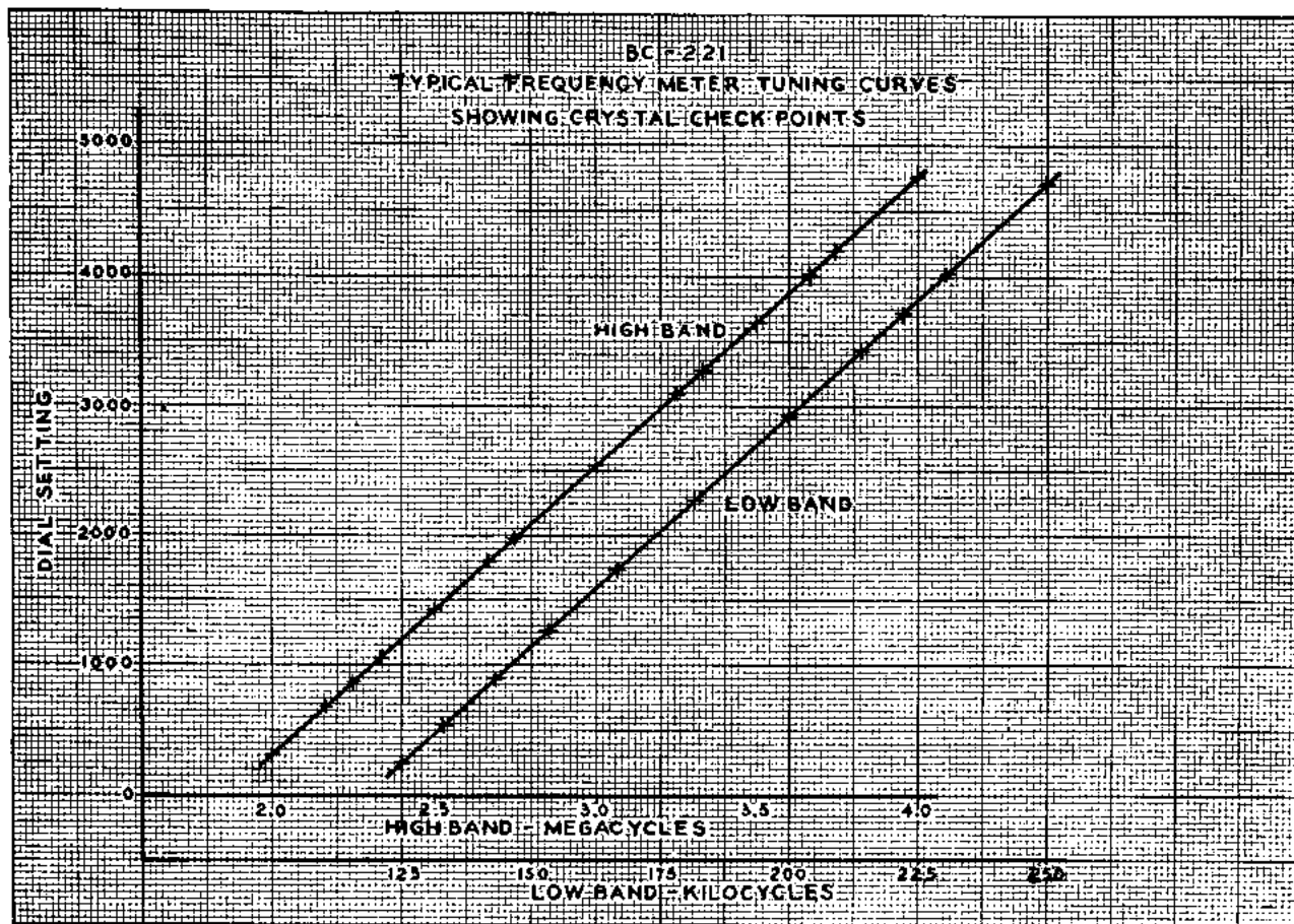
Figure 16. Frequency Meter BC-221-(8), typical frequency meter tuning curves.
