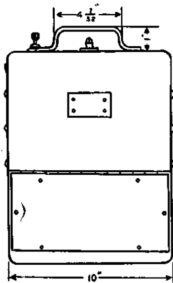
Figure 26. Frequency Meter BC-221-(3), typical dimensions, metal cabinet (subject to slight variations.)
